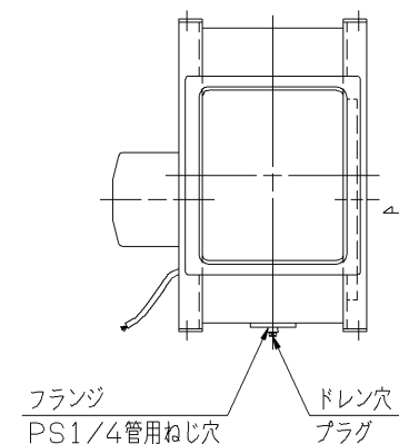
Aカラ見 VIEW FROM A
